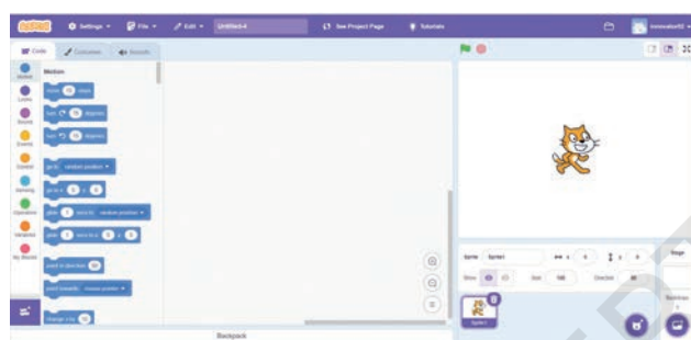
Figure 4.2: Scratch interface
